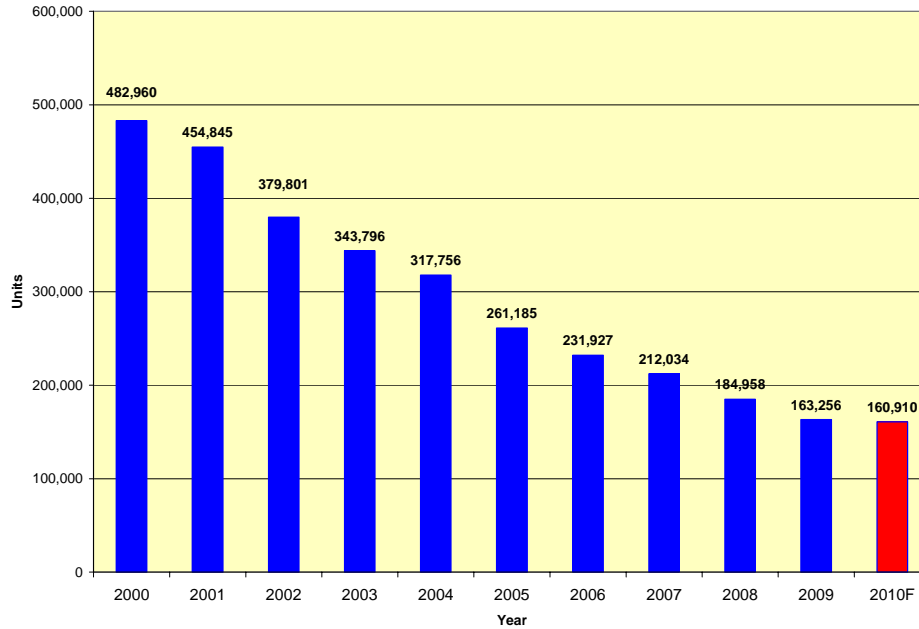
Binoculars - Historical Trends and Forecast
