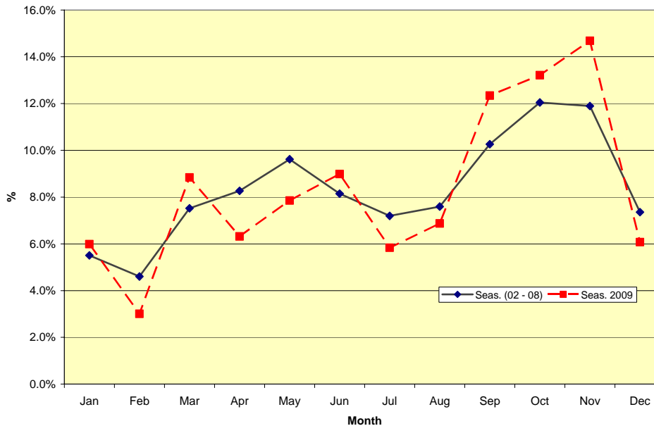
Binoculars Seasonality 2002 - 2008 vs. 2009 rolling average
